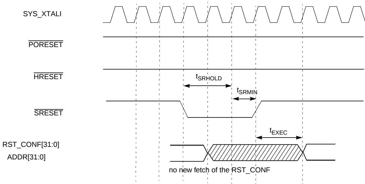
Figure 7. SRESET Behavior
