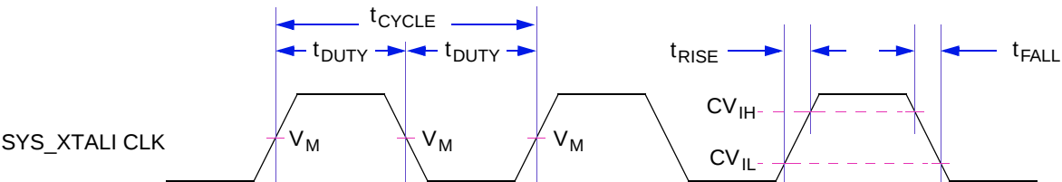
Figure 3. Timing Diagram—SYS_XTALI
