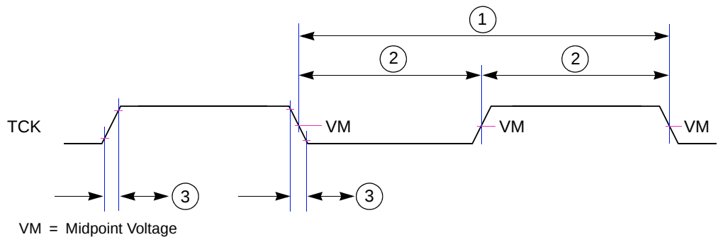
Figure 54. Timing Diagram – JTAG Clock Input
