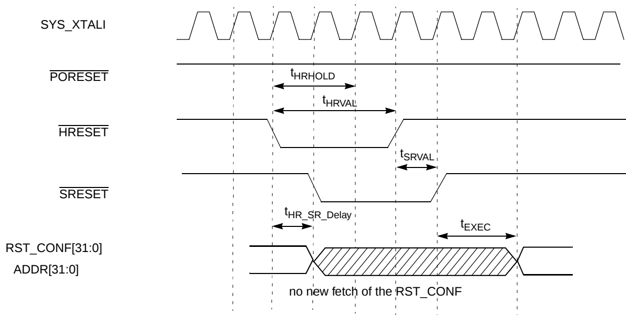
Figure 6. HRESET Behavior
