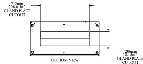
BOTTOM VIEW
