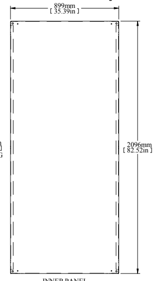
INNER PANEL
