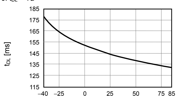
6. t_{DL} - T_a
