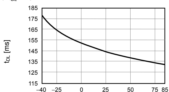
6. t_{DL} - T_a
