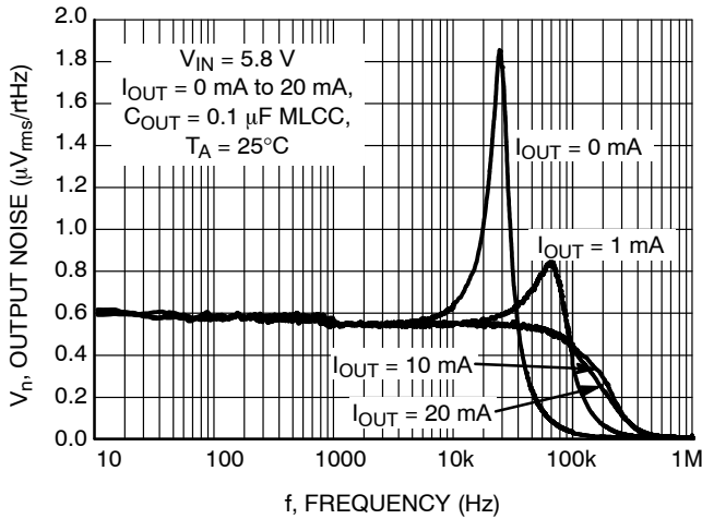
Figure 18. Output Voltage Noise 10 Hz – 1 MHz C_{OUT} = 0.1\text{ }\mu\text{F}
