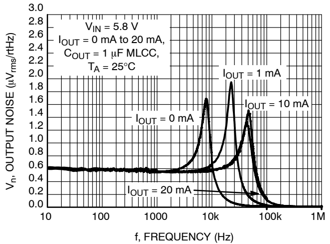
Figure 19. Output Voltage Noise 10 Hz – 1 MHz C_{OUT} = 1\text{ }\mu\text{F}
