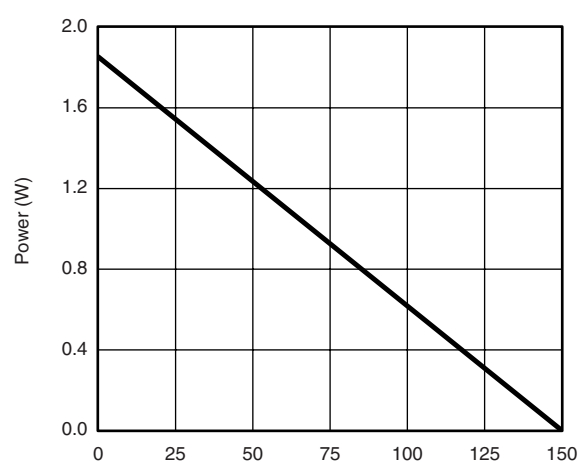
Power, Junction-to-Ambient
