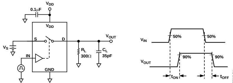
Figure 13. Switching Times
