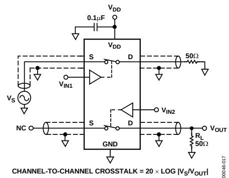
Figure 16. Channel-to-Channel Crosstalk
