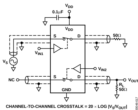
Figure 16. Channel-to-Channel Crosstalk
