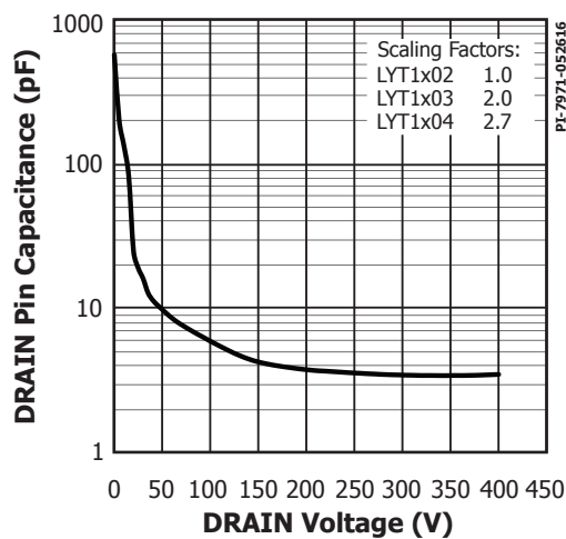
Figure 2. DRAIN Pin Capacitance vs. DRAIN Pin Voltage.
