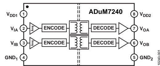
Figure 1. ADuM7240
