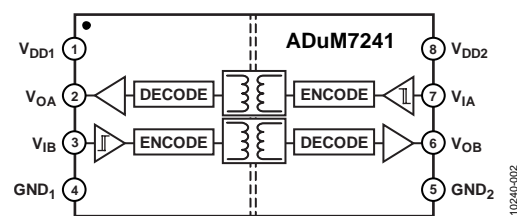
Figure 2. ADuM7241
