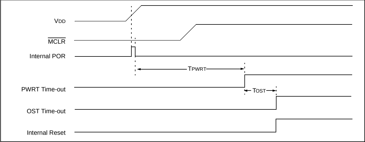
FIGURE 16-5: TIME-OUT SEQUENCE ON POWER-UP (DELAYED \overline{\text{MCLR}} ): CASE 2
