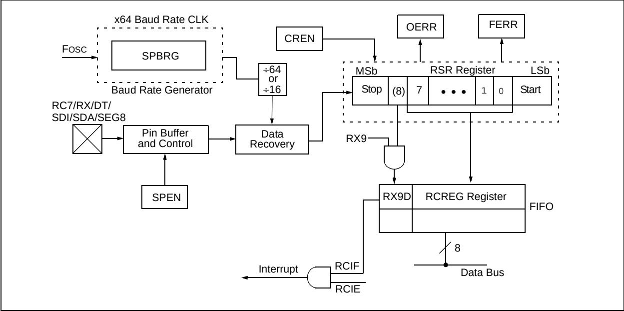
FIGURE 11-5: ASYNCHRONOUS RECEPTION
