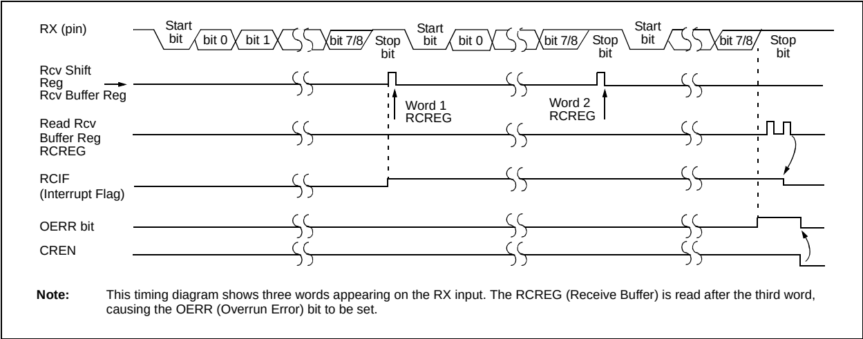
FIGURE 11-5: ASYNCHRONOUS RECEPTION
