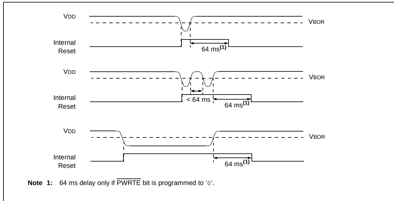
FIGURE 16-3: BROWN-OUT SITUATIONS
