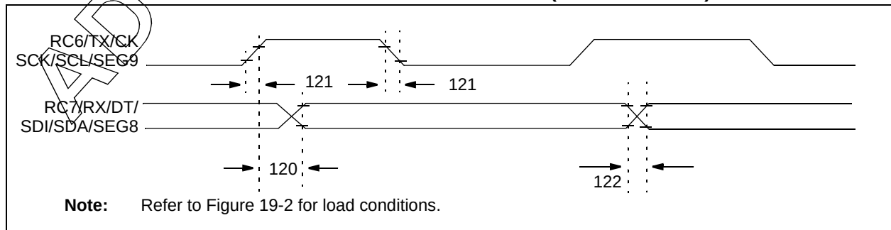
FIGURE 19-8: USART SYNCHRONOUS TRANSMISSION (MASTER/S�AVE) TIMING
