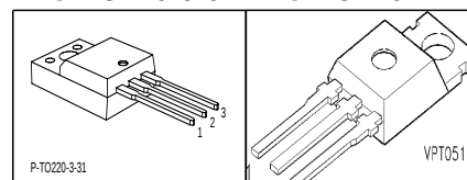
PG-TO220-3-31 PG-TO220
