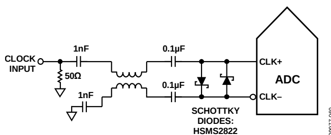
Figure 53. Balun-Coupled Differential Clock (Up to 1 GHz)
