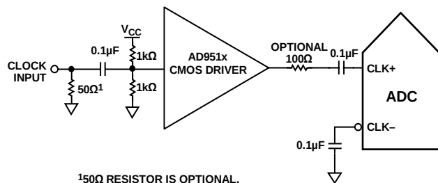
Figure 56. Single-Ended 1.8 V CMOS Input Clock (Up to 200 MHz)
