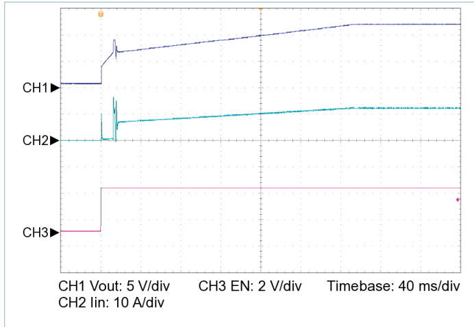
Figure 15 — Startup from EN, V_{IN} = 28\text{ V} , C_{OUT\_EXT} = 10000\text{ }\mu\text{F} , R_{LOAD} = 0.450\text{ }\Omega
