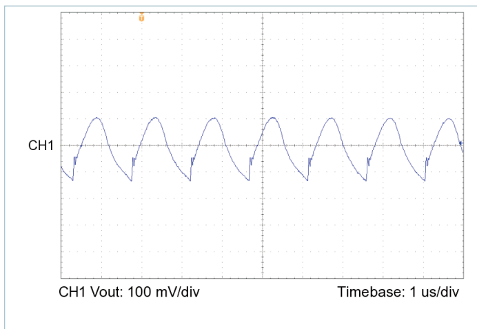
Figure 17 — Output voltage ripple, V_{IN} = 28\text{ V} , V_{OUT} = 12.0\text{ V} , C_{OUT\_EXT} = 1000\text{ }\mu\text{F} , R_{LOAD} = 0.450\text{ }\Omega
