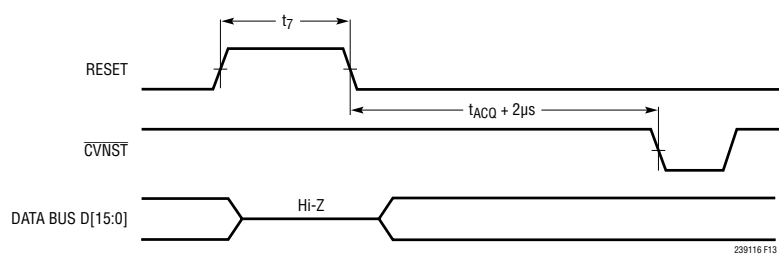
Figure 13. RESET Pin Timing
