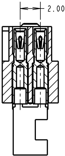
SECTION X-X
