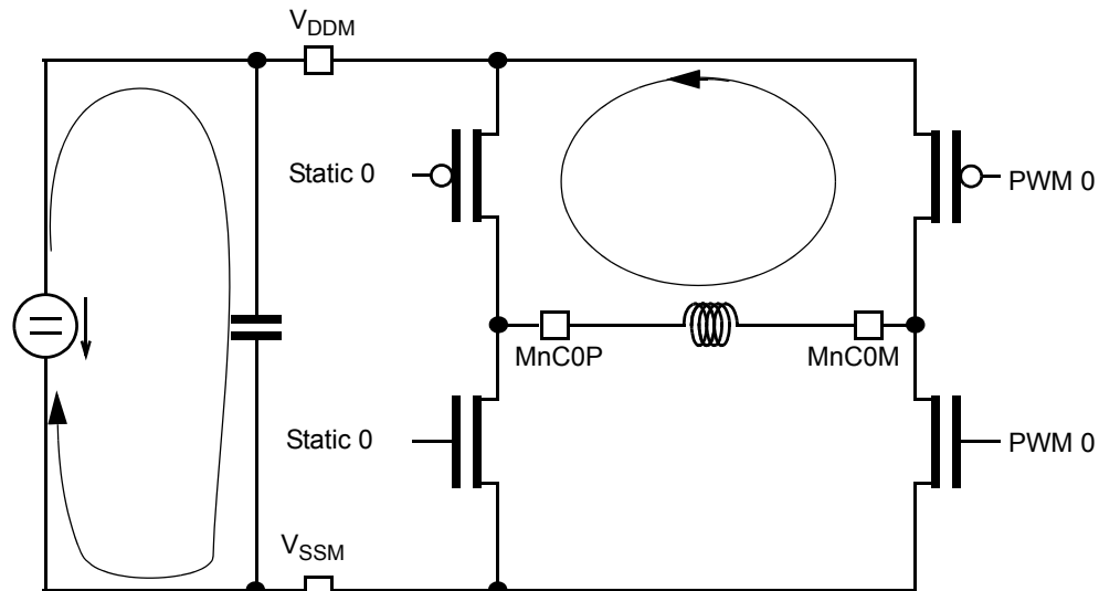
Figure 16-13. PWM Passive Phase, RECIRC = 0, S = 0
