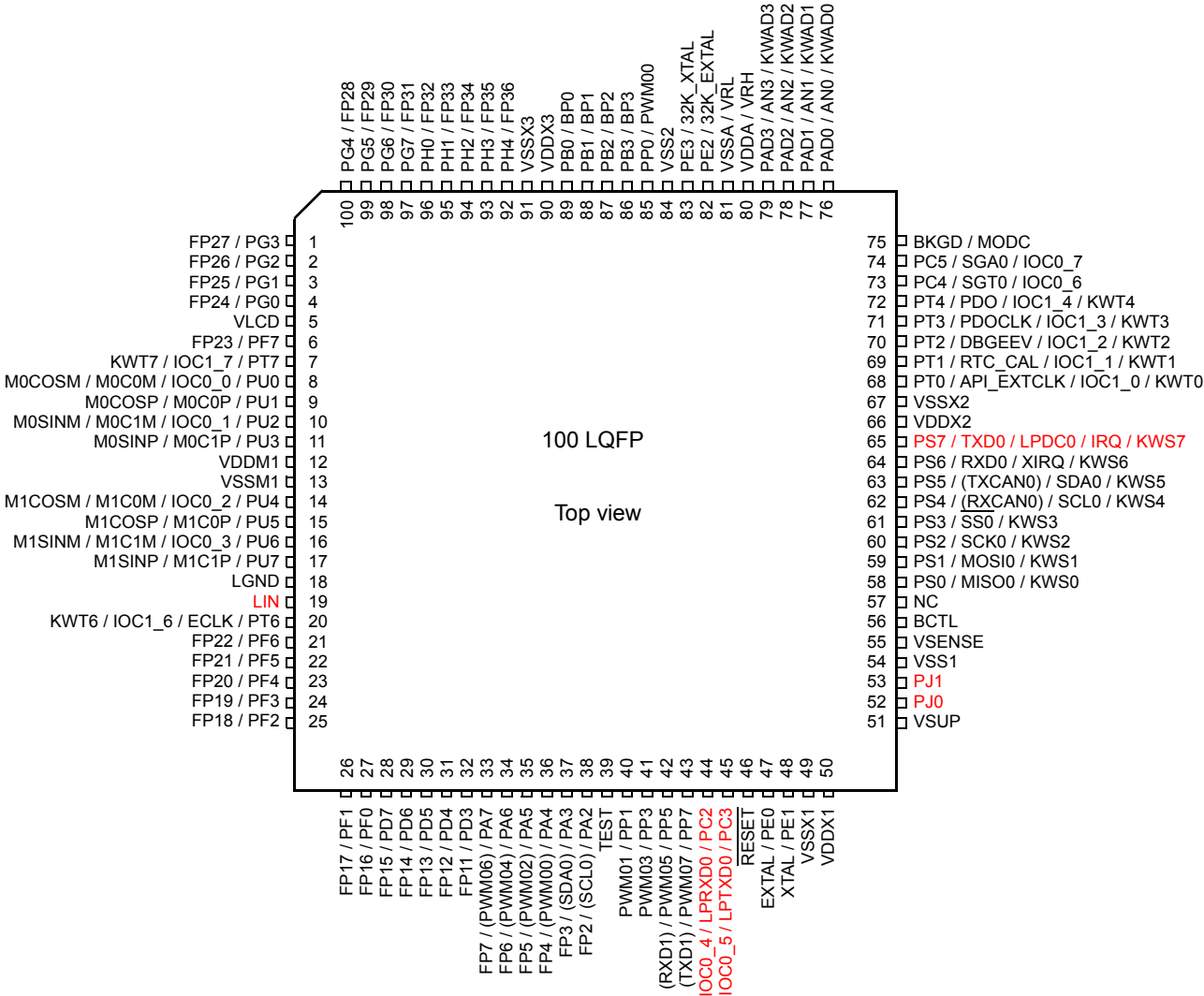
Figure 1-6. MC9S12ZVHL 100-pin LQFP pin out
