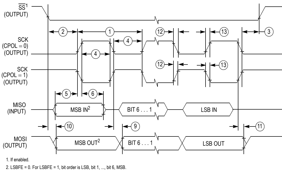
Figure L-1. SPI Master Timing (CPHA=0)
