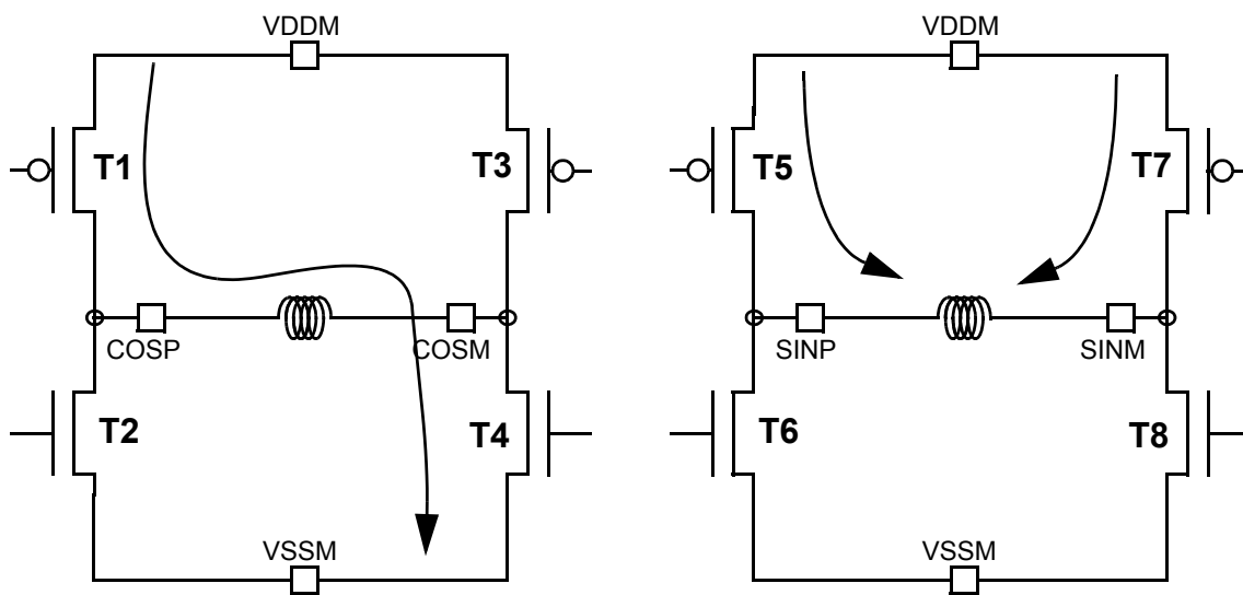
Figure 17-11. Current Flow when STEP = 0, DCOIL = 1, ITG = 0, RCIR = 0
