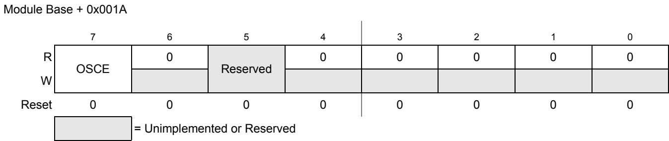
Figure 7-31. S12CPMU_UHV_V5 Oscillator Register (CPMUOSC)
