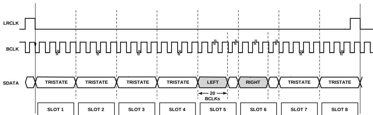
Figure 17. TDM8 Channel 5 to Channel 6, CONFIG Pin Tied to IOVDD Through a 47 kΩ Resistor
