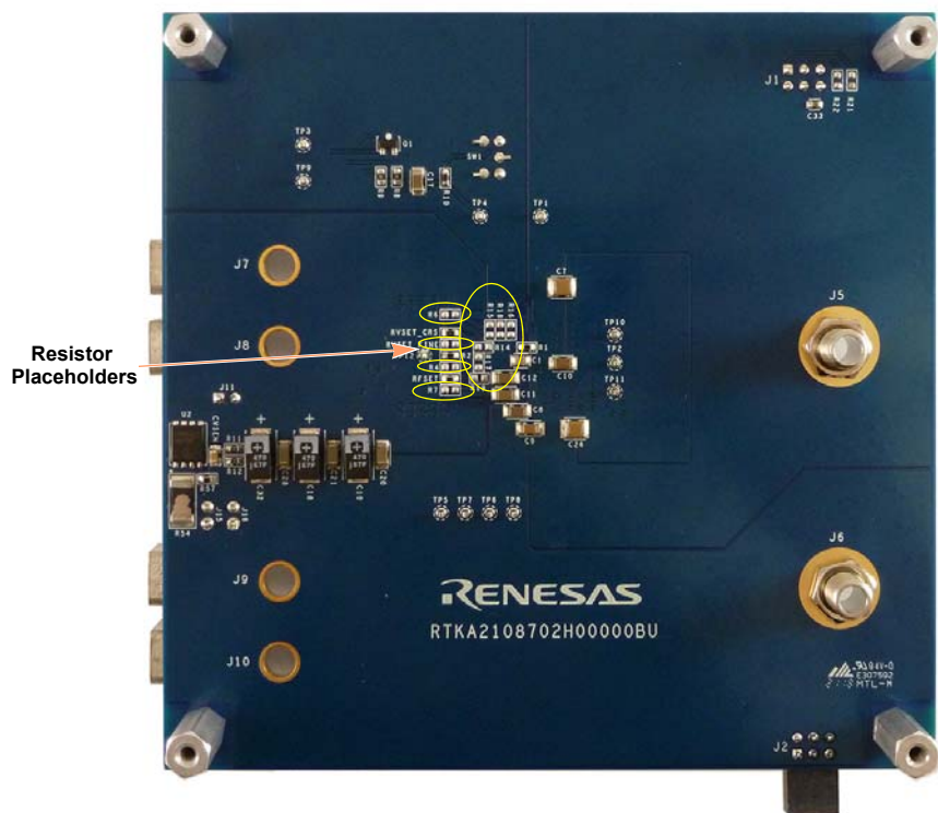
Figure 6. RTKA2108702H00000BU Evaluation Board (Bottom Side)
