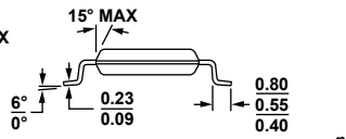
Figure 45. 8-Lead Mini Small Outline Package [MSOP] (RM-8)
