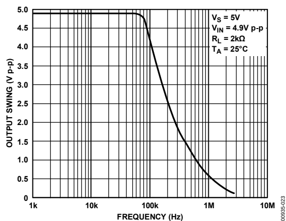
Figure 24. Closed-Loop Output Voltage Swing vs. Frequency
