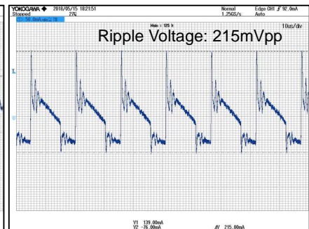
Figure 20. VOUT Ripple Voltage.3 V_{IN}=100Vac , I_{OUT}=1500mA CH1: VOUT 50mV/div, 10 \mu s /div
