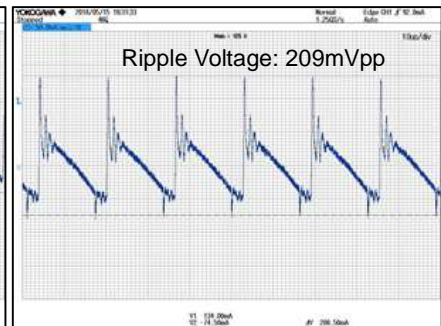
Figure 23. VOUT Ripple Voltage.6 V_{IN}=230Vac , I_{OUT}=1500mA CH1: VOUT 50mV/div, 10 \mu s /div
