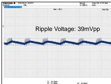
Figure 18. VOUT Ripple Voltage.1 V_{IN}=100Vac , I_{OUT}=10mA CH1: VOUT 50mV/div, 1000 \mu s /div
