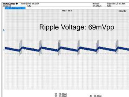
Figure 21. VOUT Ripple Voltage.4 V_{IN}=230Vac , I_{OUT}=10mA CH1: VOUT 50mV/div, 1000 \mu s /div
