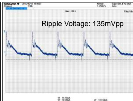
Figure 22. VOUT Ripple Voltage.5 V_{IN}=230Vac , I_{OUT}=500mA CH1: VOUT 50mV/div, 10 \mu s /div
