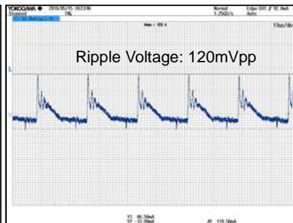
Figure 19. VOUT Ripple Voltage.2 V_{IN}=100Vac , I_{OUT}=500mA CH1: VOUT 50mV/div, 10 \mu s /div
