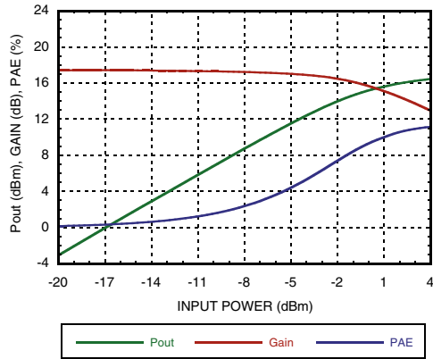
Power Compression @ 12 GHz [1]
