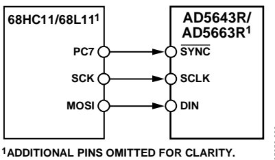
Figure 57. AD5623R/AD5643R/AD5663R to 68HC11/68L11 Interface
