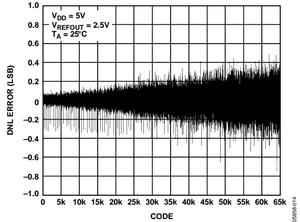
Figure 13. DNL—AD5663R-5
