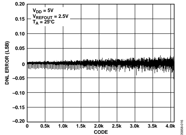
Figure 15. DNL—AD5623R-5
