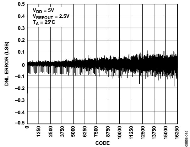
Figure 14. DNL—AD5643R-5
