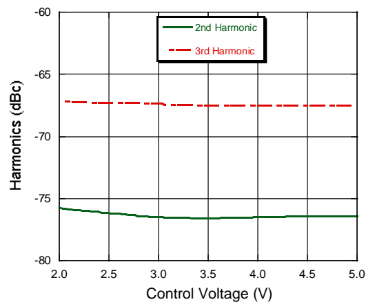
Harmonics vs. Control Voltage, 1 GHz
