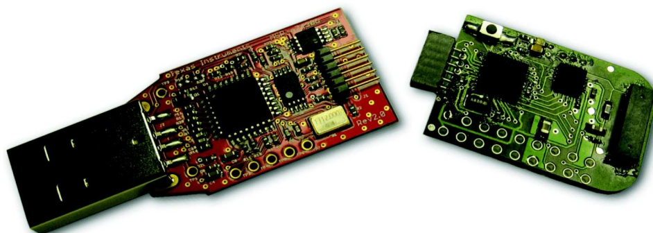
Figure 1. eZ430-TMS37157
