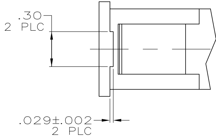
DETAIL T
