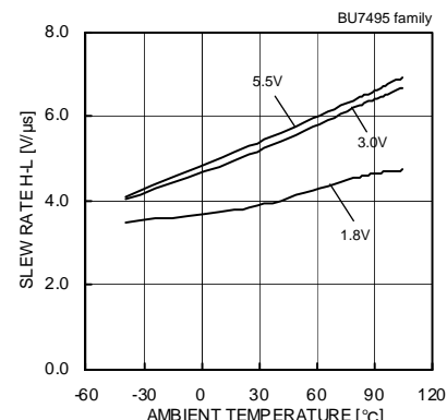
Slew Rate H-L – Ambient Temperature
