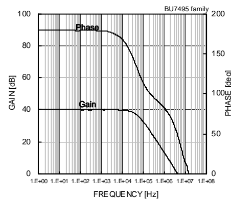
Voltage Gain – Frequency
