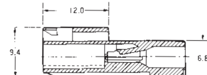
Section X-X
