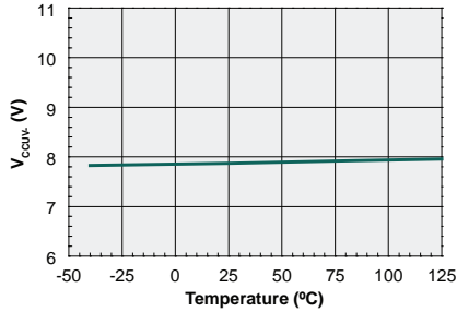
V_{CCUV-} vs. Temperature
