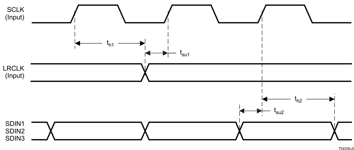
Figure 3-1. Slave Mode Serial Data Interface Timing
