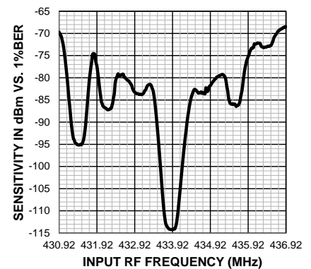
434MHz Selectivity at 1.625KHz Bandwidth
