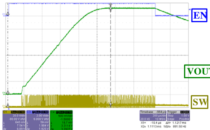
Figure 10. Typical start-up with V_{IN} = 19\text{ V} , V_{OUT} = 3.3\text{ V} and I_{OUT} = 0\text{ A}
