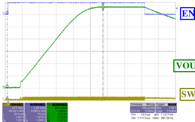
Figure 8. Typical start-up with V_{IN} = 4.5\text{ V} , V_{OUT} = 3.3\text{ V} and I_{OUT} = 0\text{ A}
