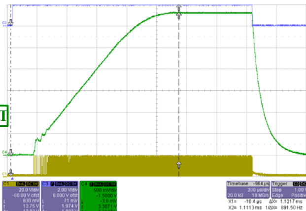
Figure 11. Typical start-up with V_{IN} = 19\text{ V} , V_{OUT} = 3.3\text{ V} and I_{OUT} = 1\text{ A}
