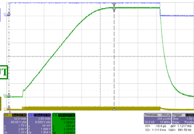
Figure 9. Typical start-up with V_{IN} = 4.5\text{ V} , V_{OUT} = 3.3\text{ V} and I_{OUT} = 1\text{ A}
