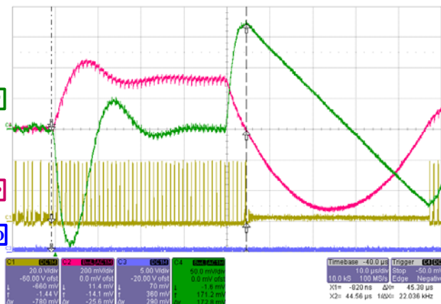
Figure 13. Load transient 0.1 A to 1.2 A, with V_{OUT} = 3.3\text{ V} and V_{IN} = 36\text{ V}
