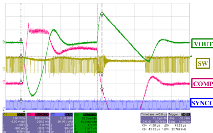
Figure 12. Load transient 0.1 A to 1.2 A, with V_{OUT} = 3.3\text{ V} and V_{IN} = 4.6\text{ V}
