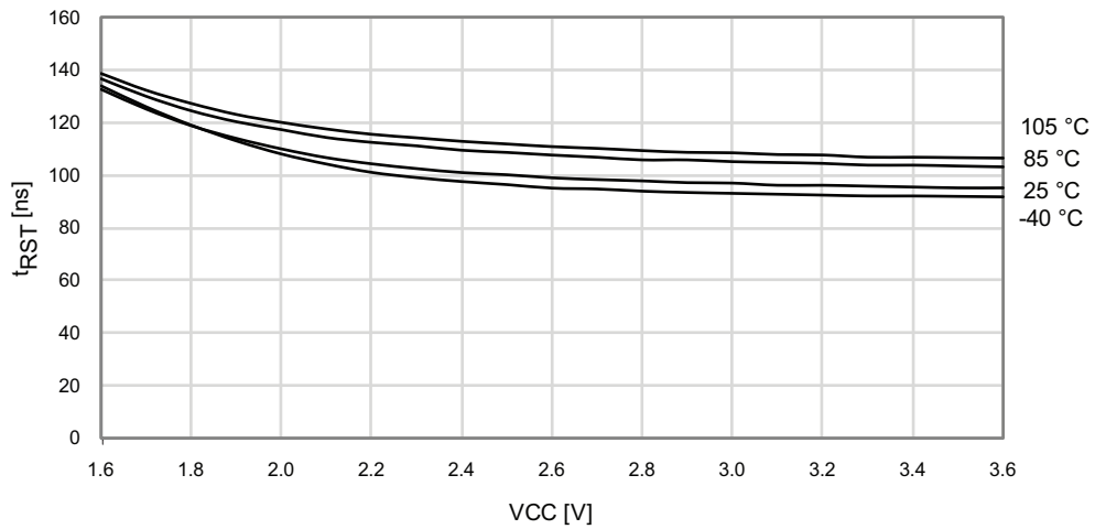
Figure 33-190. Minimum Reset Pin Pulse Width vs. V CC
