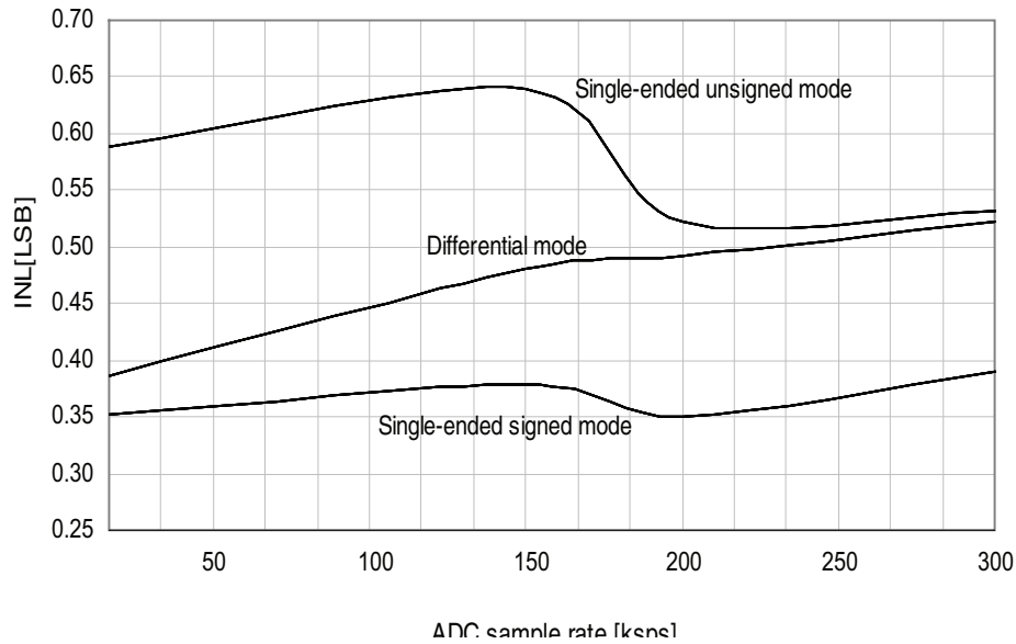
Figure 33-313. INL Error vs. Sample Rate T = 25°C, V CC = 3.6V, V REF = 3.0V external
