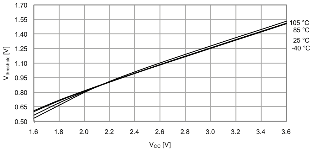
Figure 33-380. I/O Pin Input Threshold Voltage vs. V_{CC}
