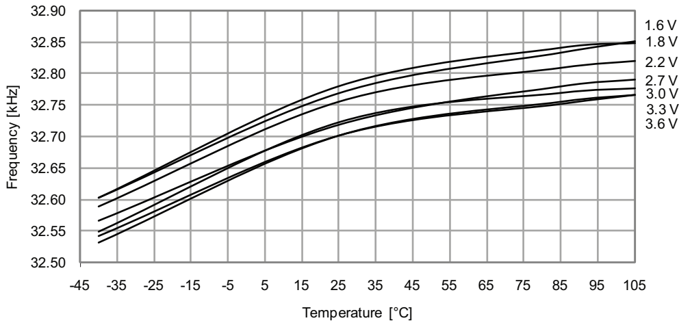
Figure 33-406. 32.768kHz Internal Oscillator Frequency vs. Temperature
