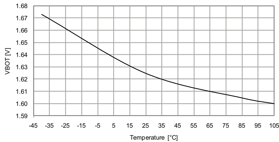
Figure 33-398. BOD Thresholds vs. Temperature BOD level = 1.6V
