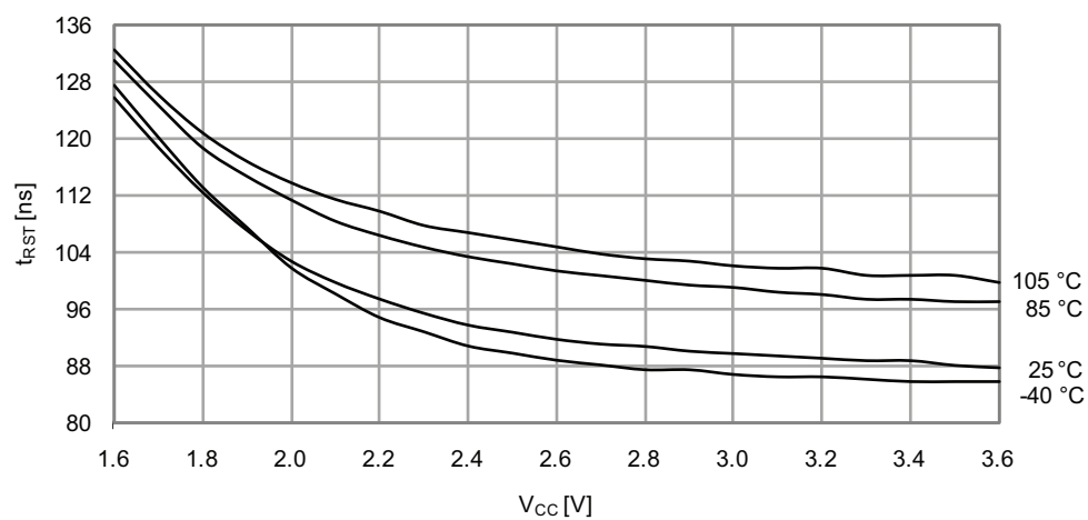
Figure 33-260. Minimum Reset Pin Pulse Width vs. V_{CC}
