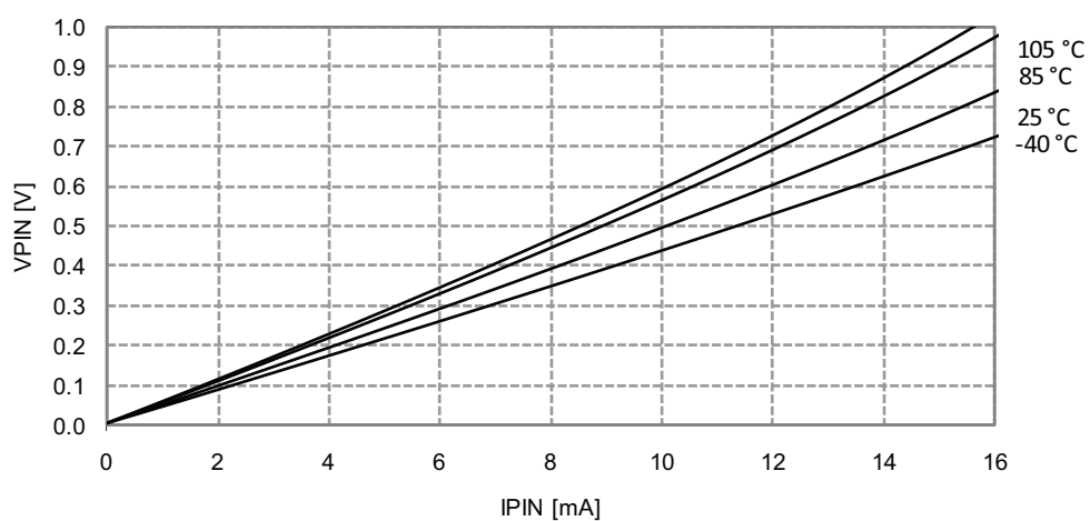
Figure 33-307. I/O Pin Output Voltage vs. Sink Current
