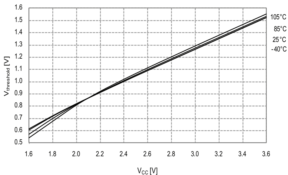
Figure 33-100. I/O Pin Input Threshold Voltage vs. V_{CC} V_{IL} I/O pin read as "0"
