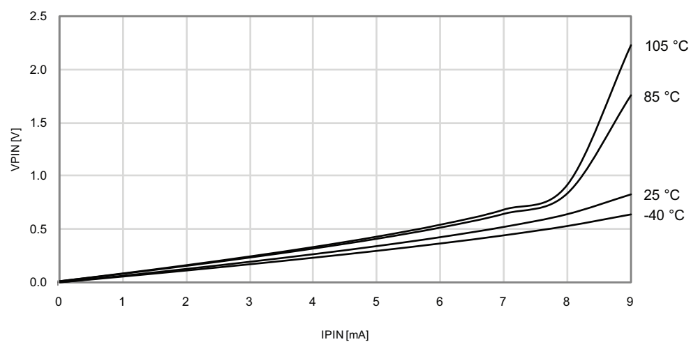
Figure 33-166. I/O Pin Output Voltage vs. Sink Current
