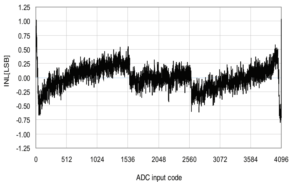
Figure 33-314. INL Error vs. Input Code
