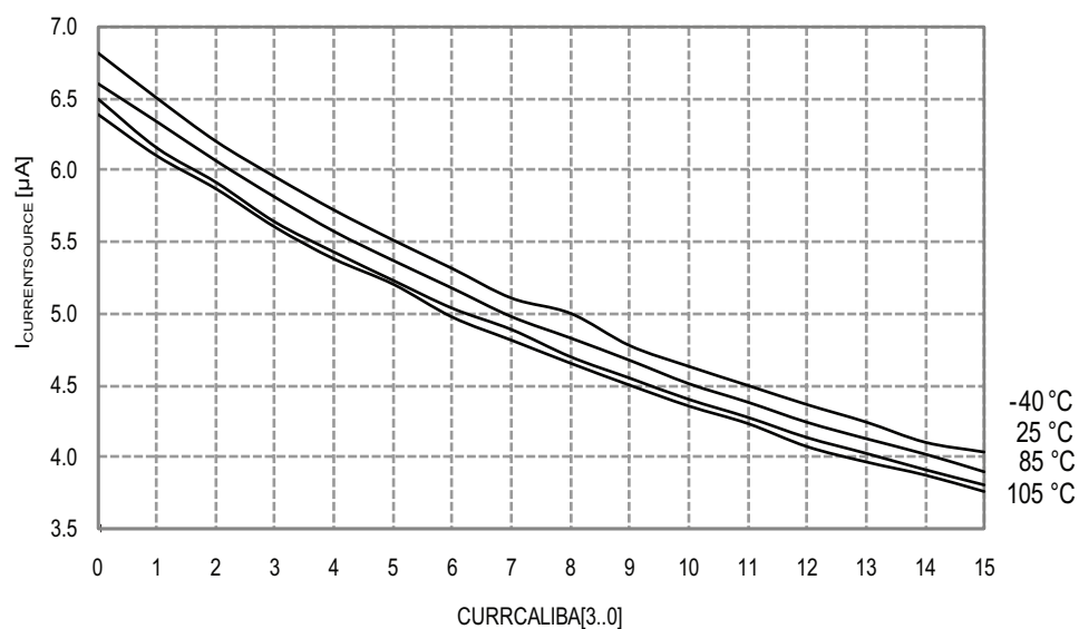
Figure 33-256. Voltage Scaler INL vs. SCALEFAC
