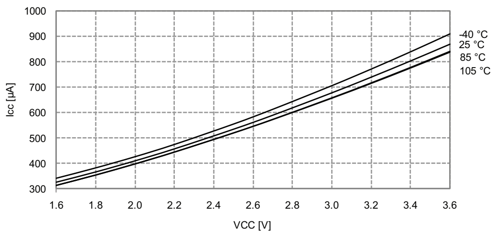
Figure 33-295. Idle Mode Supply Current vs. V_{CC} f_{SYS} = 32\text{MHz} internal oscillator prescaled to 8MHz
