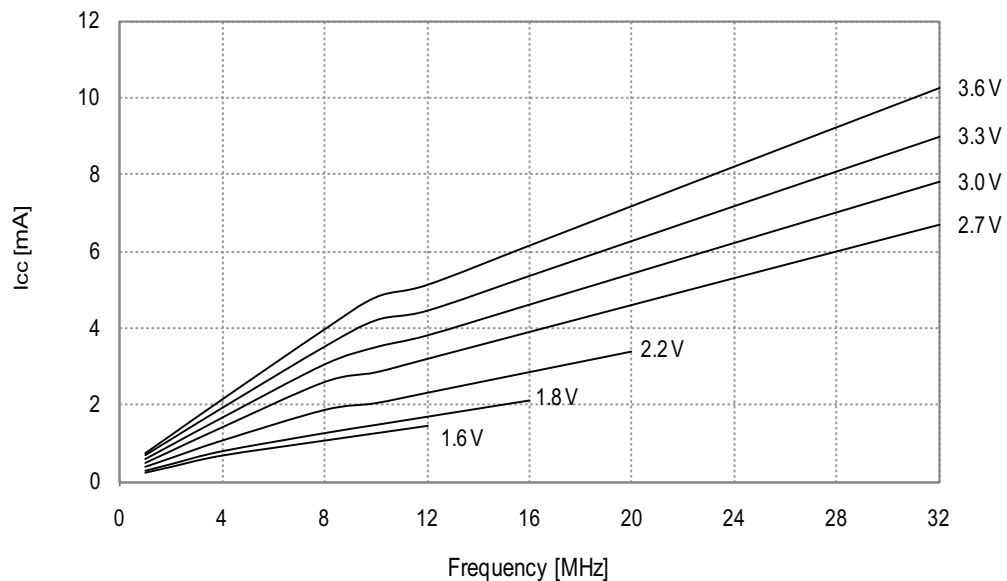
Figure 33-73. Active Supply Current vs. Frequency
