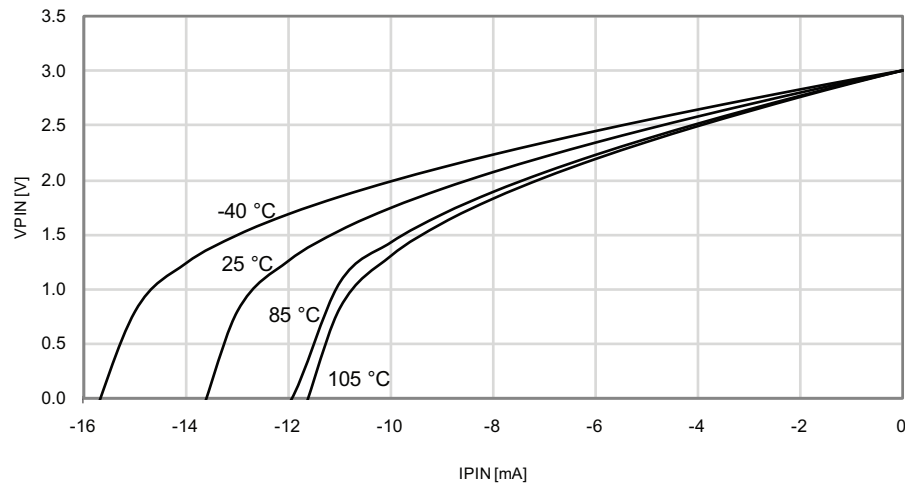
Figure 33-164. I/O Pin Output Voltage vs. Source Current V_{CC} = 3.0V
