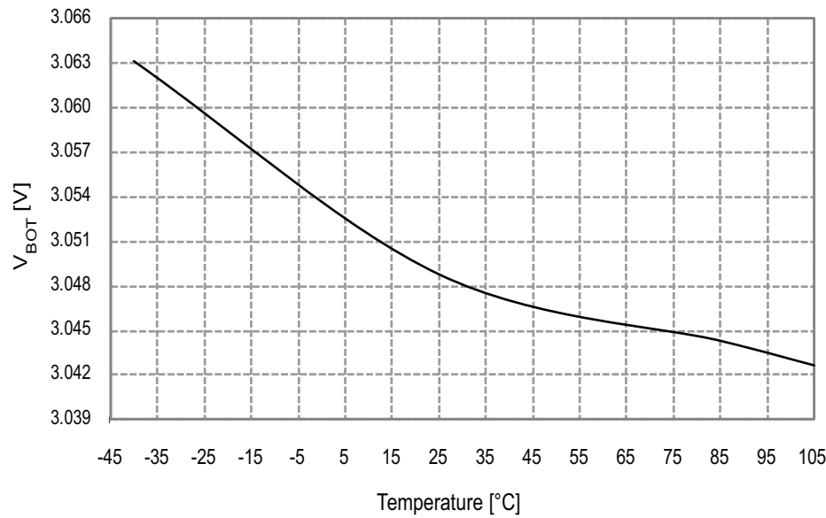
Figure 33-48. BOD Thresholds vs. Temperature BOD level = 3.0V
