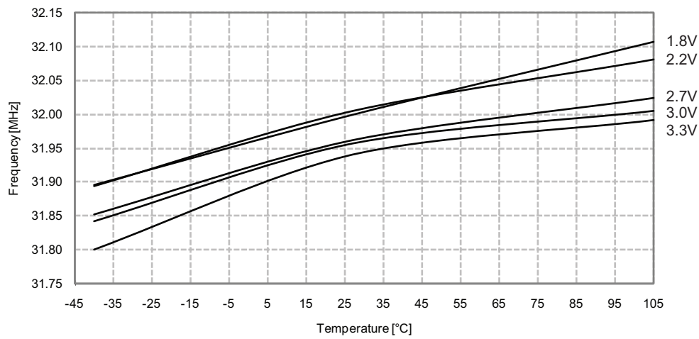
Figure 33-272. 32MHz Internal Oscillator Frequency vs. Temperature DPLL enabled, from the 32.768kHz internal oscillator
