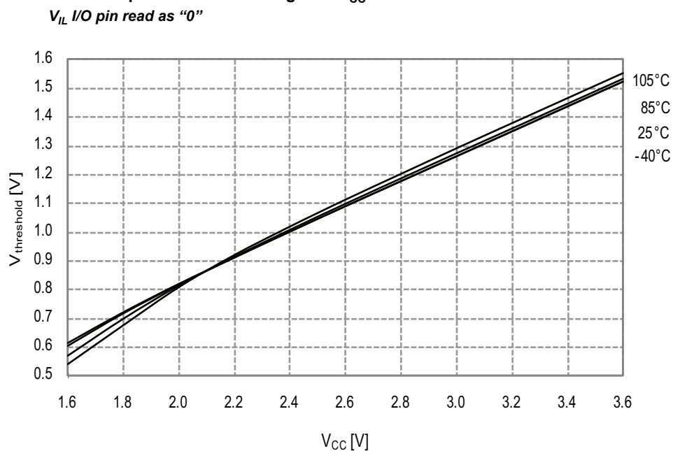
Figure 33-29. I/O Pin Input Threshold Voltage vs. V_{CC}
