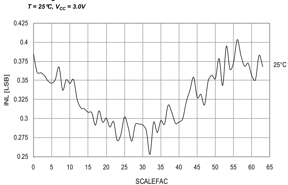
Figure 33-186. Voltage Scaler INL vs. SCALEFAC
