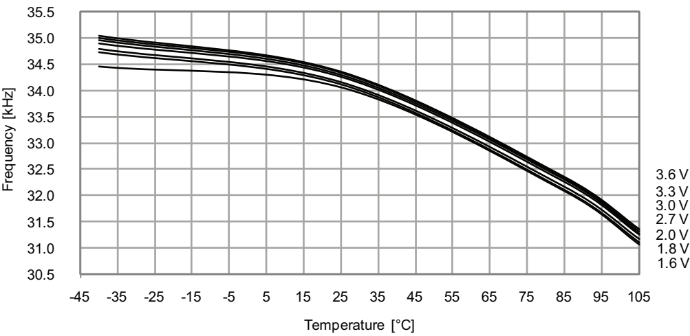
Figure 33-405. Ultra Low-Power Internal Oscillator Frequency vs. Temperature
