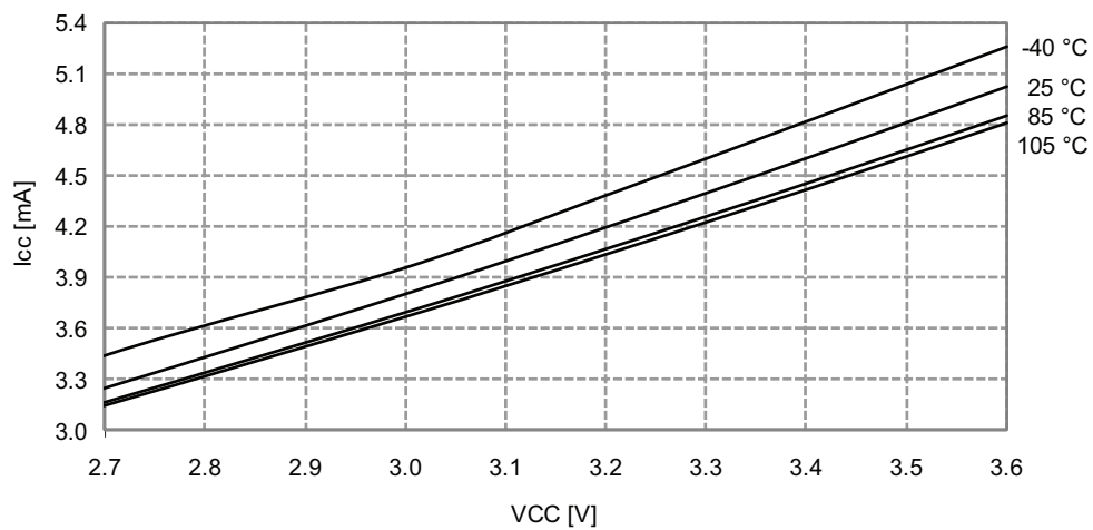
Figure 33-296. Idle Mode Current vs. V_{CC} f_{SYS} = 32\text{MHz} internal oscillator
