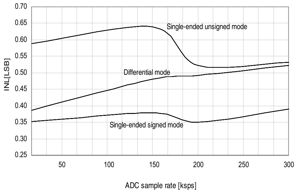
Figure 33-103. INL Error vs. Sample Rate T = 25^{\circ}\text{C} , V_{CC} = 3.6\text{V} , V_{REF} = 3.0\text{V} external
