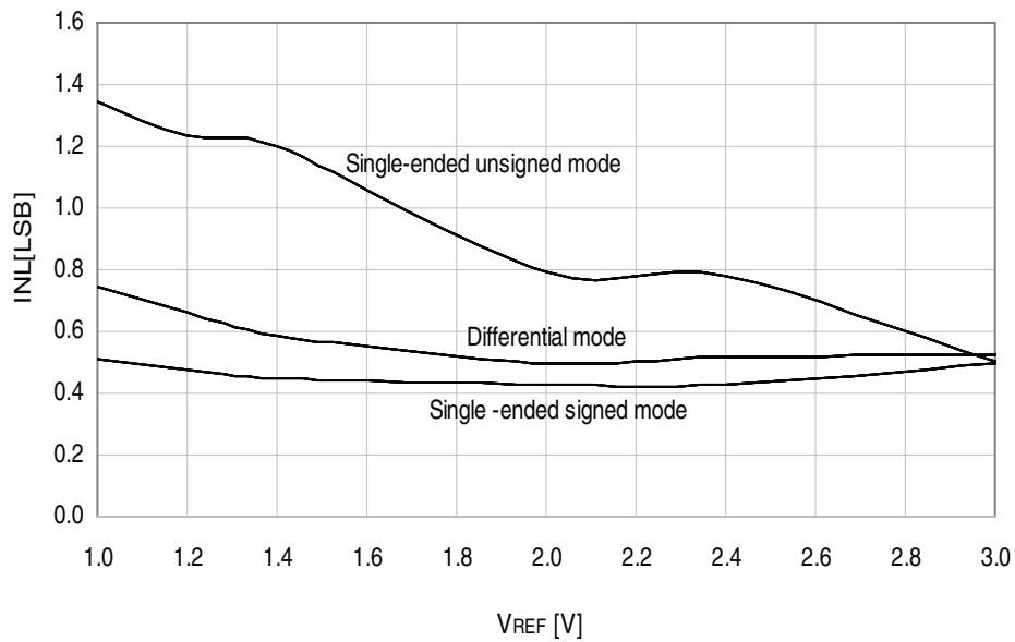
Figure 33-102. INL Error vs. External V_{REF} T = 25^{\circ}\text{C} , V_{CC} = 3.6\text{V} , external reference
