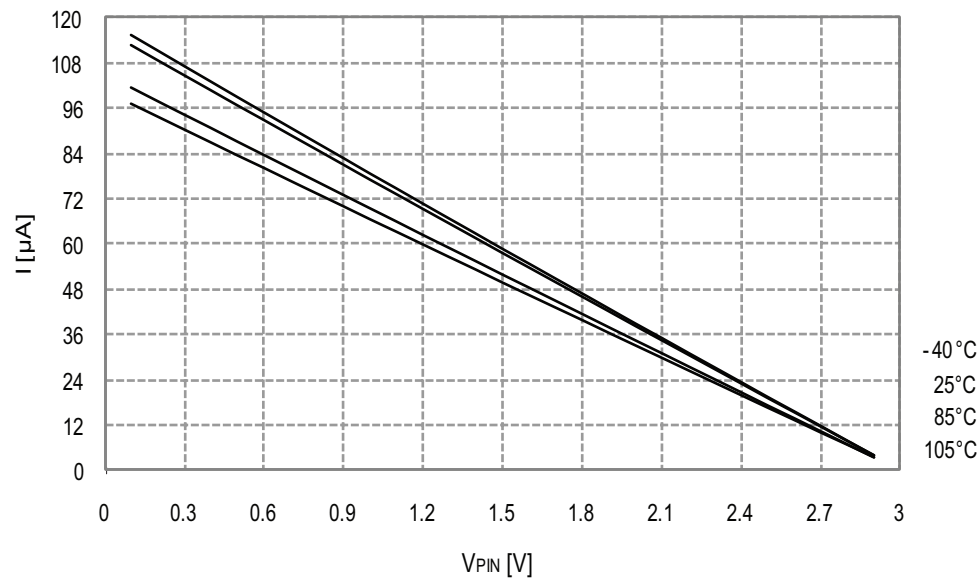
Figure 33-20. I/O Pin Pull-up Resistor Current vs. Input Voltage V_{CC} = 3.0V
