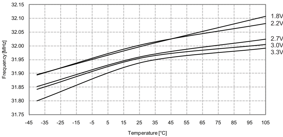
Figure 33-412. 32MHz Internal Oscillator Frequency vs. Temperature DPLL enabled, from the 32.768kHz internal oscillator
