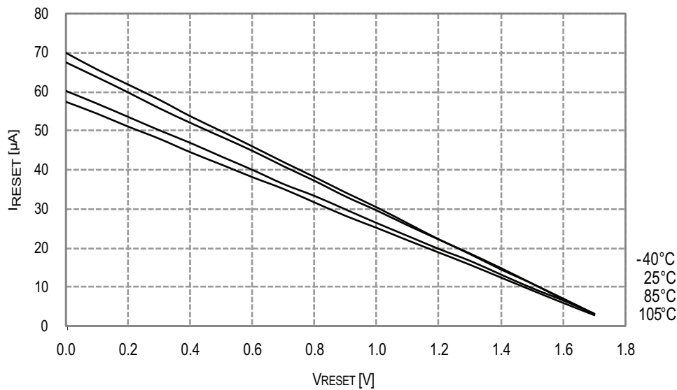
Figure 33-50. Reset Pin Pull-up Resistor Current vs. Reset Pin Voltage
