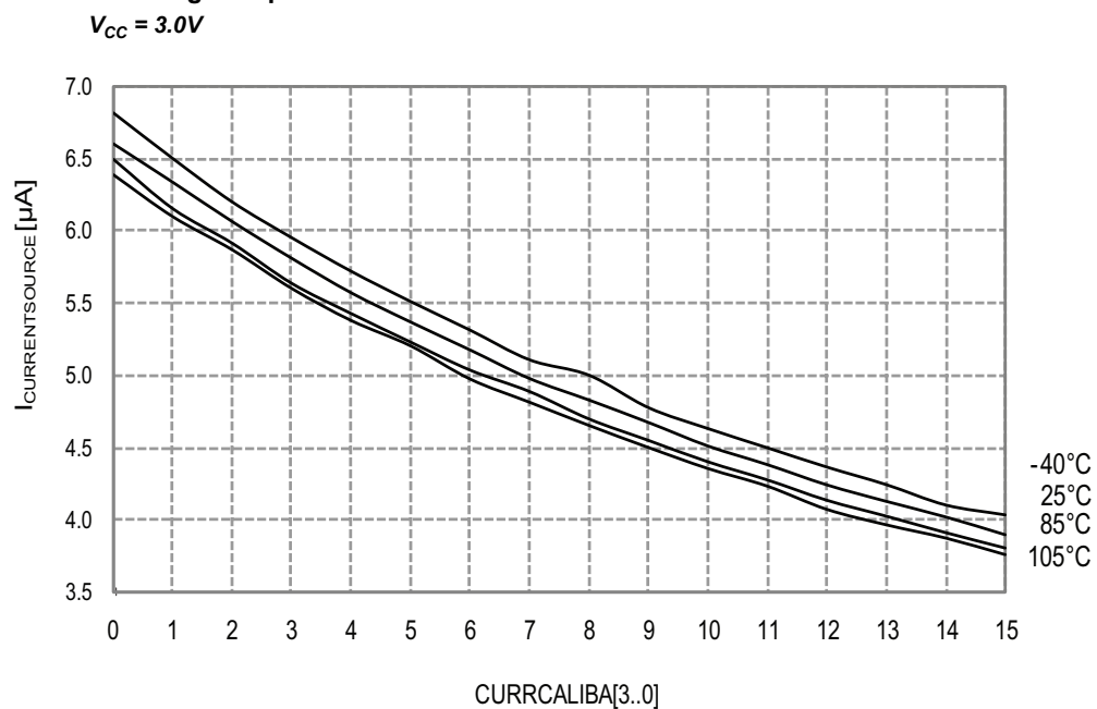
Figure 33-185. Analog Comparator Current Source vs. Calibration Value
