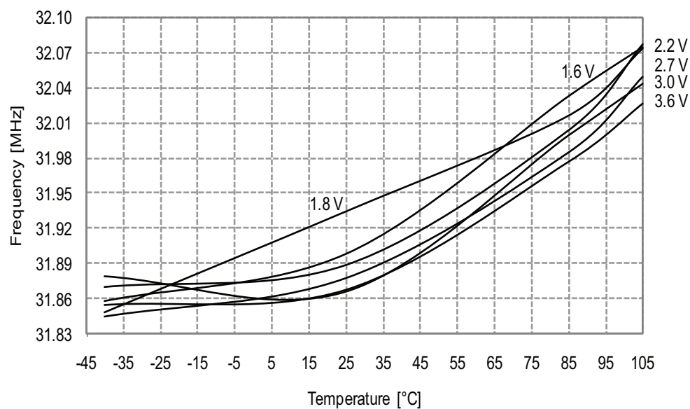
Figure 33-132. 32MHz Internal Oscillator Frequency vs. Temperature DFLL enabled, from the 32.768kHz internal oscillator
