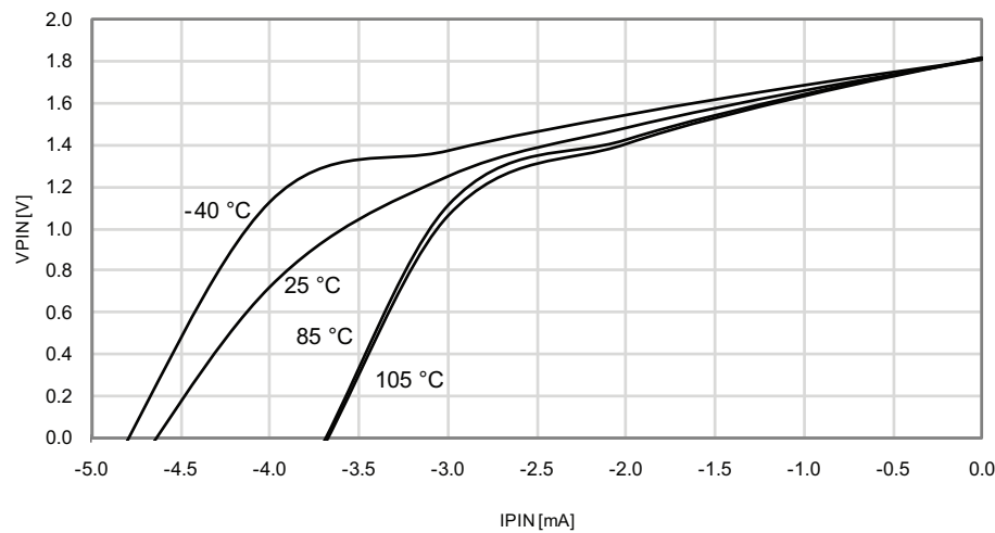
Figure 33-163. I/O Pin Output Voltage vs. Source Current V_{CC} = 1.8V
