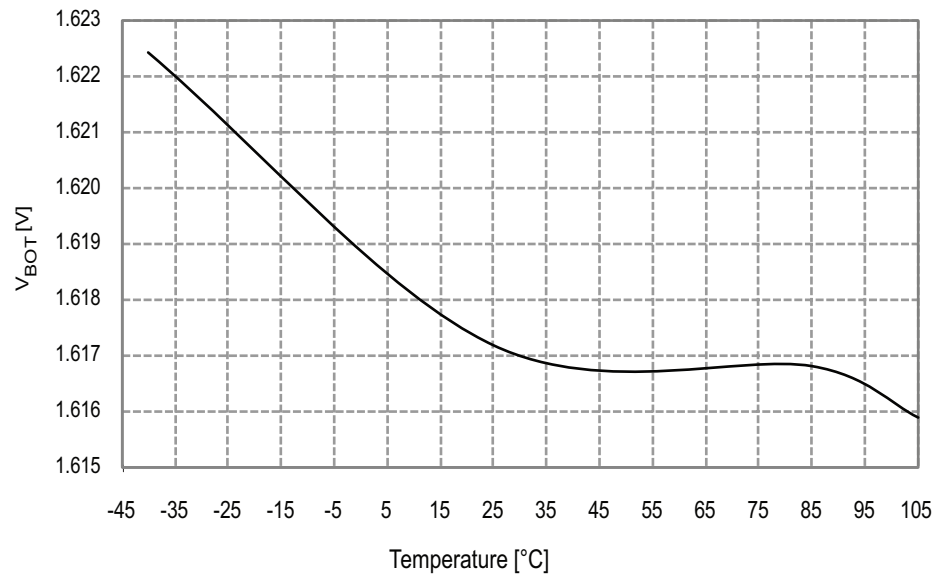
Figure 33-47. BOD Thresholds vs. Temperature BOD level = 1.6V
