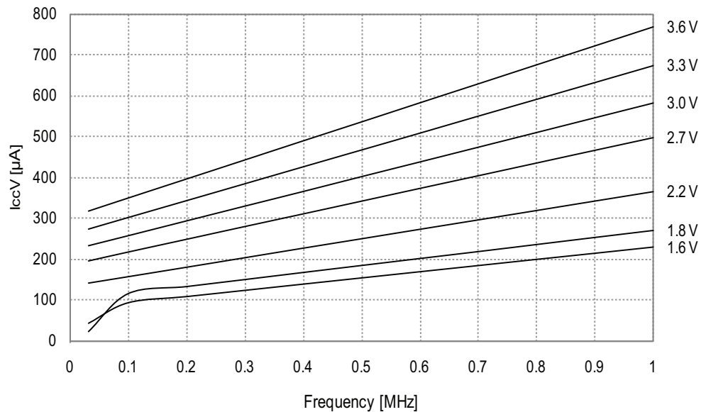
Figure 33-72. Active Supply Current vs. Frequency
