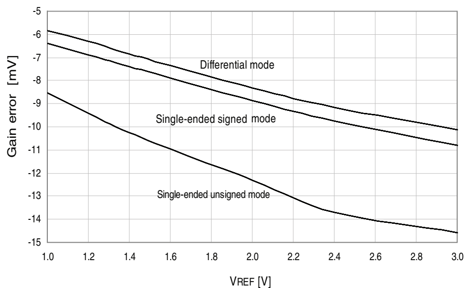
Figure 33-388. Gain Error vs. V_{REF} T = 25^{\circ}\text{C} , V_{CC} = 3.6\text{V} , ADC sample rate = 300ksps
