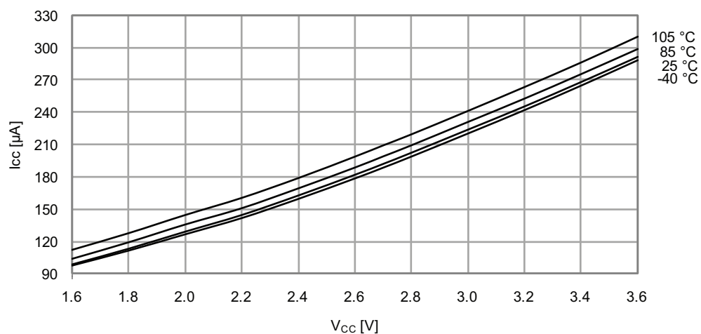
Figure 33-363. Idle Mode Supply Current vs. V_{CC}
