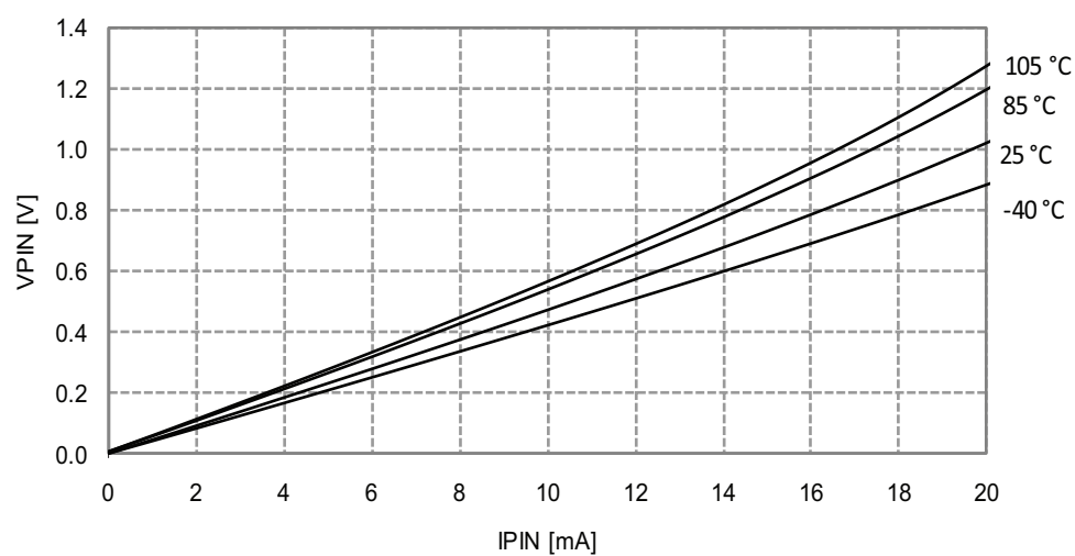
Figure 33-378. I/O Pin Output Voltage vs. Sink Current
