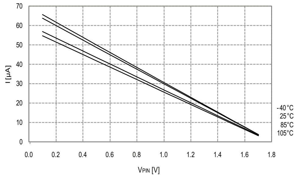
Figure 33-20. I/O Pin Pull-up Resistor Current vs. Input Voltage V_{CC} = 3.0V
