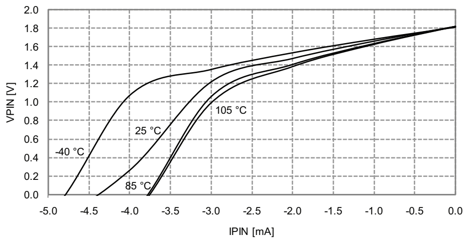
Figure 33-303. I/O Pin Output Voltage vs. Source Current
