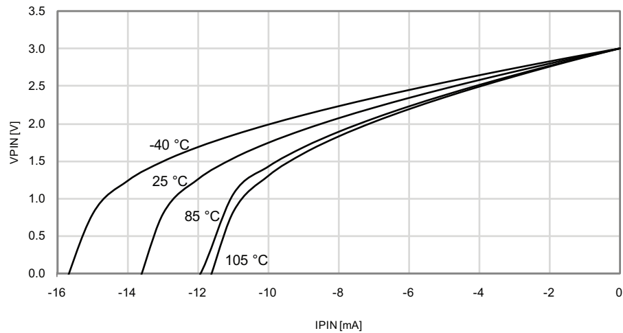
Figure 33-164. I/O Pin Output Voltage vs. Source Current V_{CC} = 3.0V
