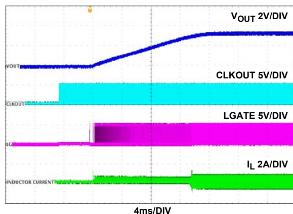
FIGURE 12. CCM START-UP WAVEFORMS: V_{OUT} , I_{L} , I_{GATE} , CLKOUT , I_O = 0A
