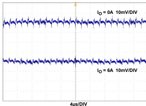
FIGURE 10. OUTPUT RIPPLE, MODE = CCM
