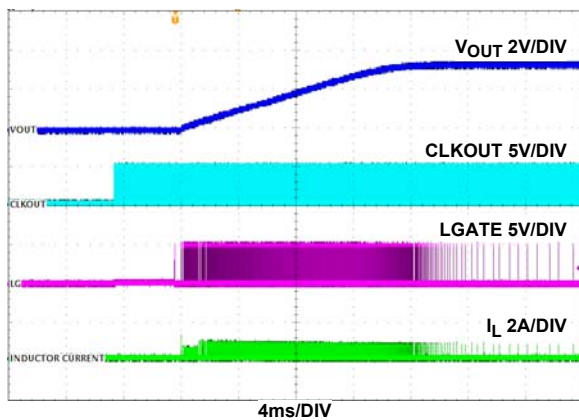
FIGURE 13. DEM START-UP WAVEFORMS: V_{OUT} , I_{L} , I_{GATE} , CLKOUT , I_O = 0A
