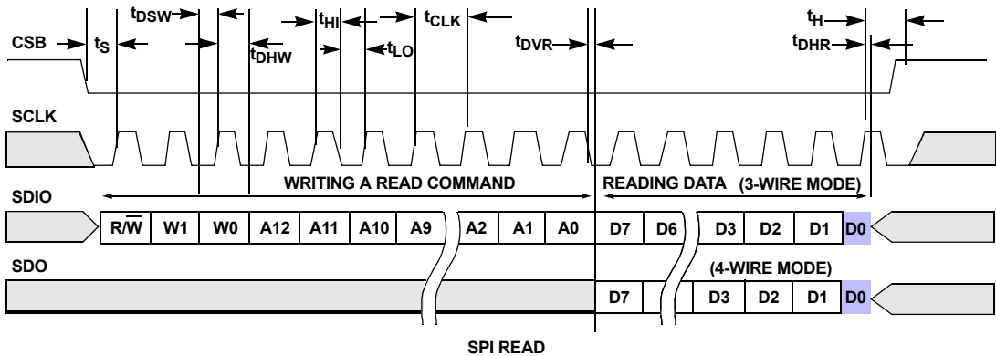
FIGURE 39. SPI READ
