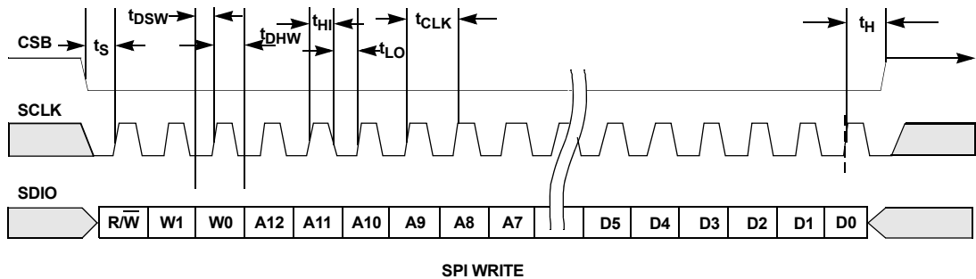
FIGURE 38. SPI WRITE
