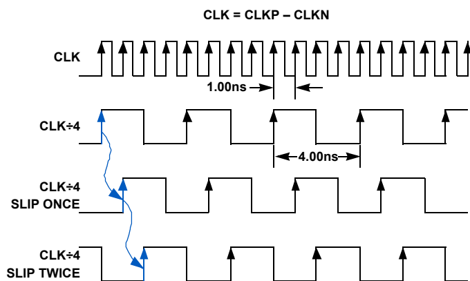
FIGURE 42. PHASE SLIP: CLK÷4 MODE, f_{\text{CLK}} = 1000\text{MHz}
